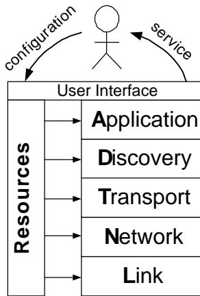
Figure 5. User-device interaction
