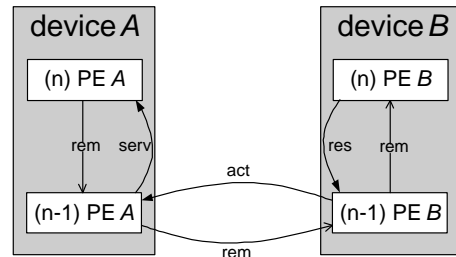
Figure 13. Hidden Cooperation
